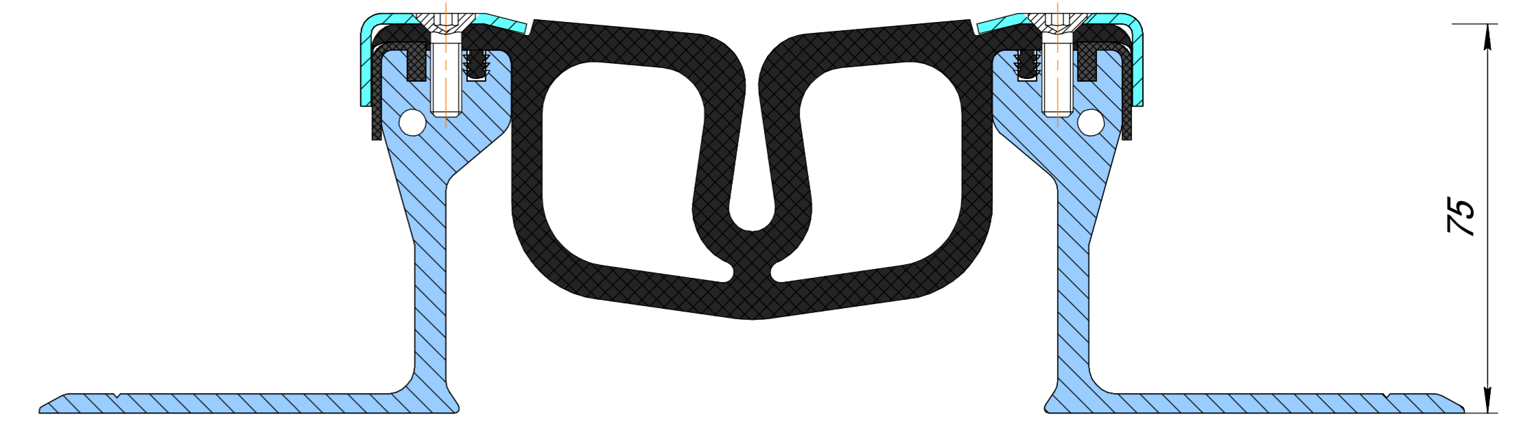
Dewmark Hydro WR 73/110/75/S
