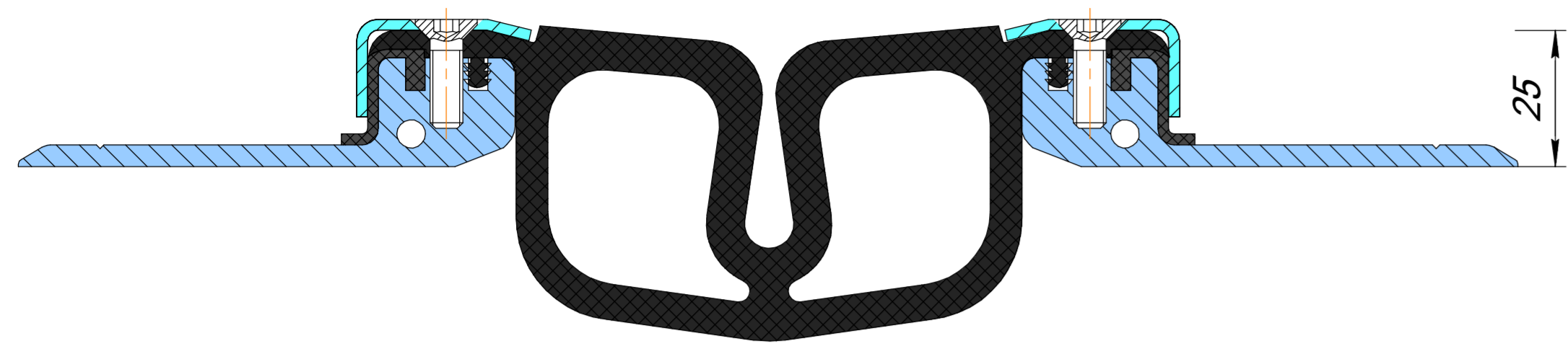
Dewmark Hydro WR 73/110/25/S
