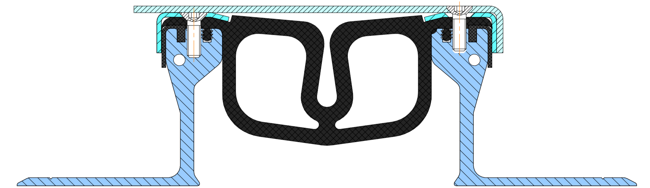
Dewmark Hydro WR 73/110/75/S/F
