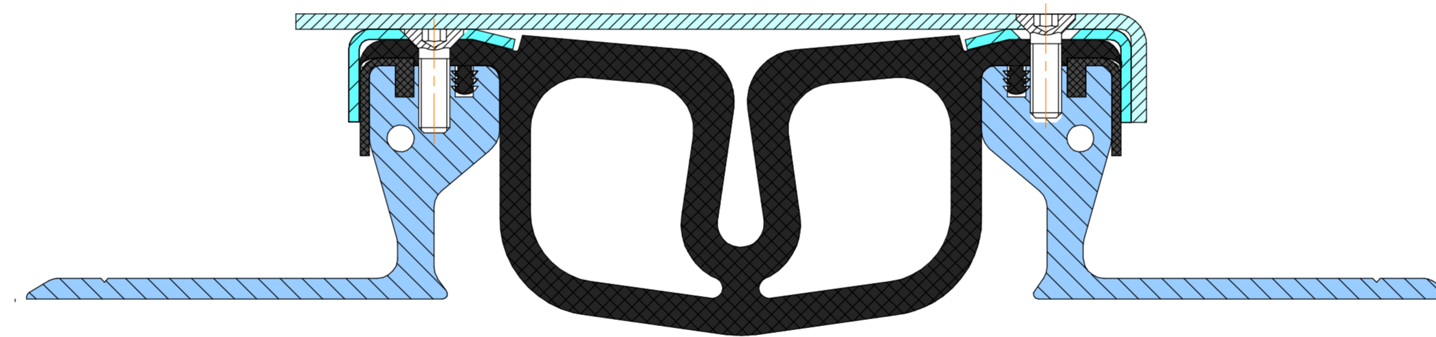
Dewmark Hydro WR 73/110/80/S/F
