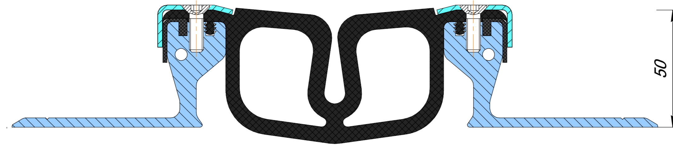
Dewmark Hydro WR 73/110/50/S
