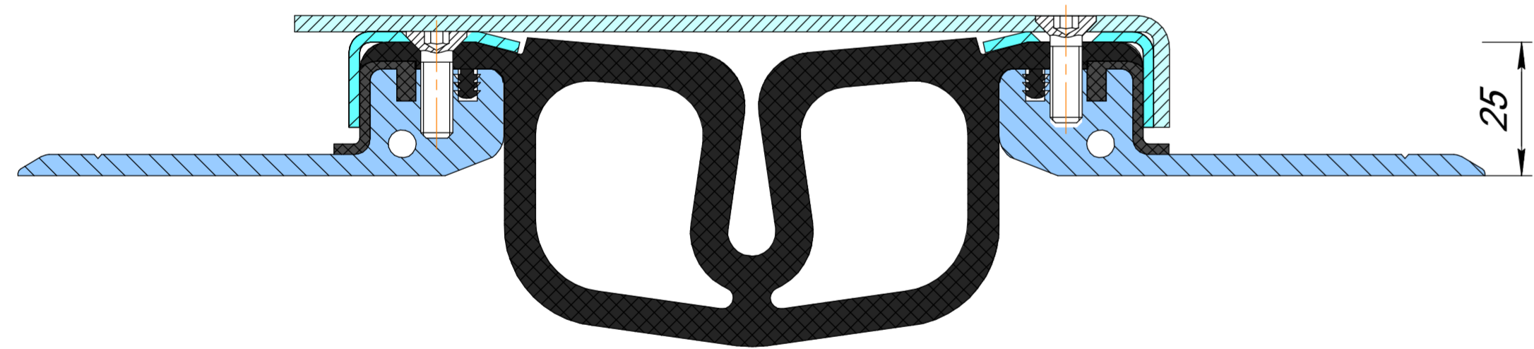
Dewmark Hydro WR 73/110/25/S/F
