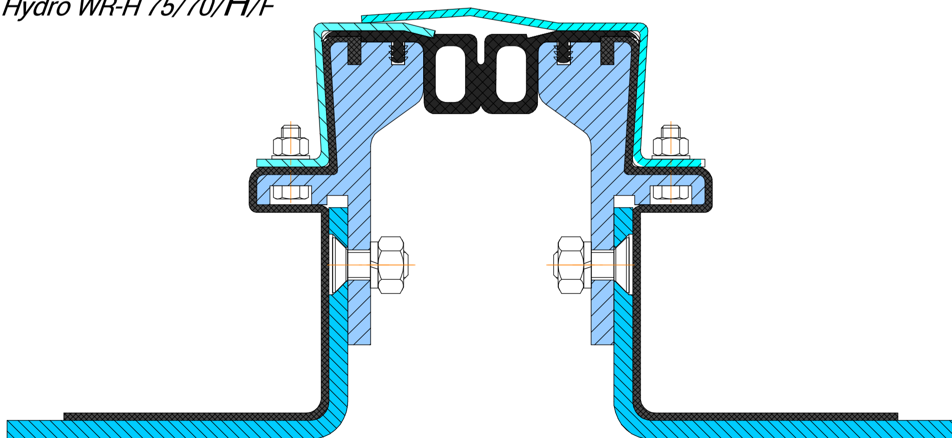
Dewmark Hydro WR-H 75/70/H/F
