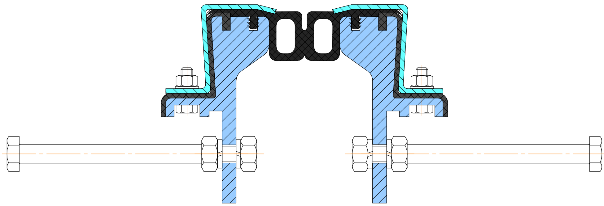
Dewmark Hydro WR 75
