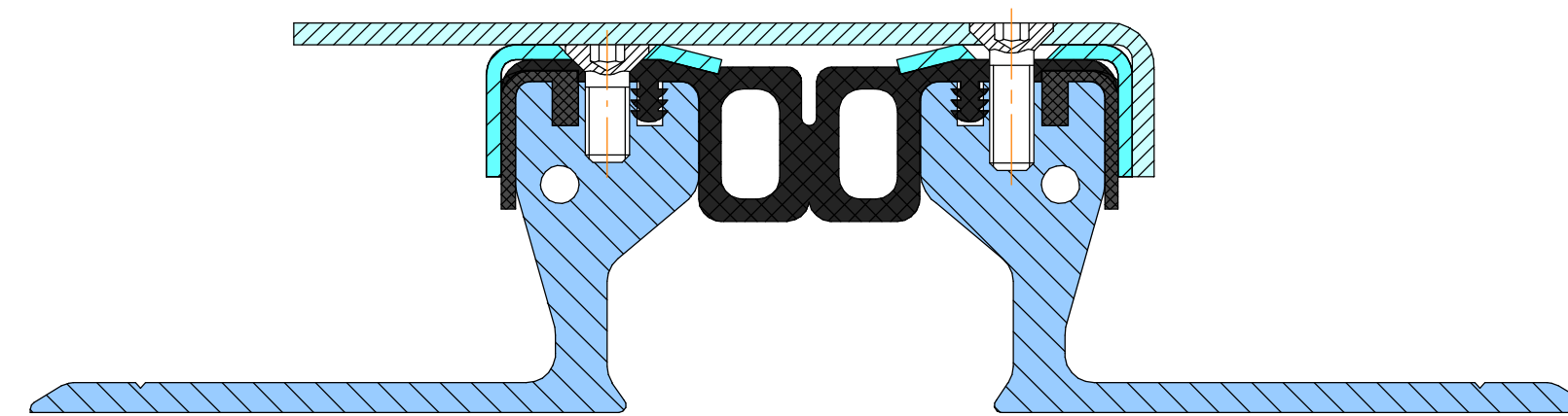
Dewmark Hydro WR 73/50/50/S/F
