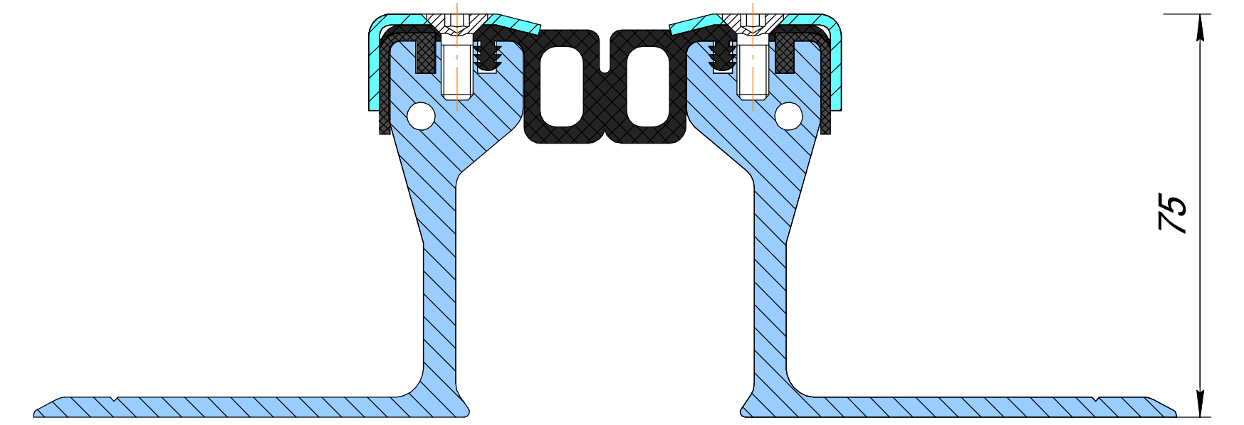
Dewmark Hydro WR 73/50/75/S
