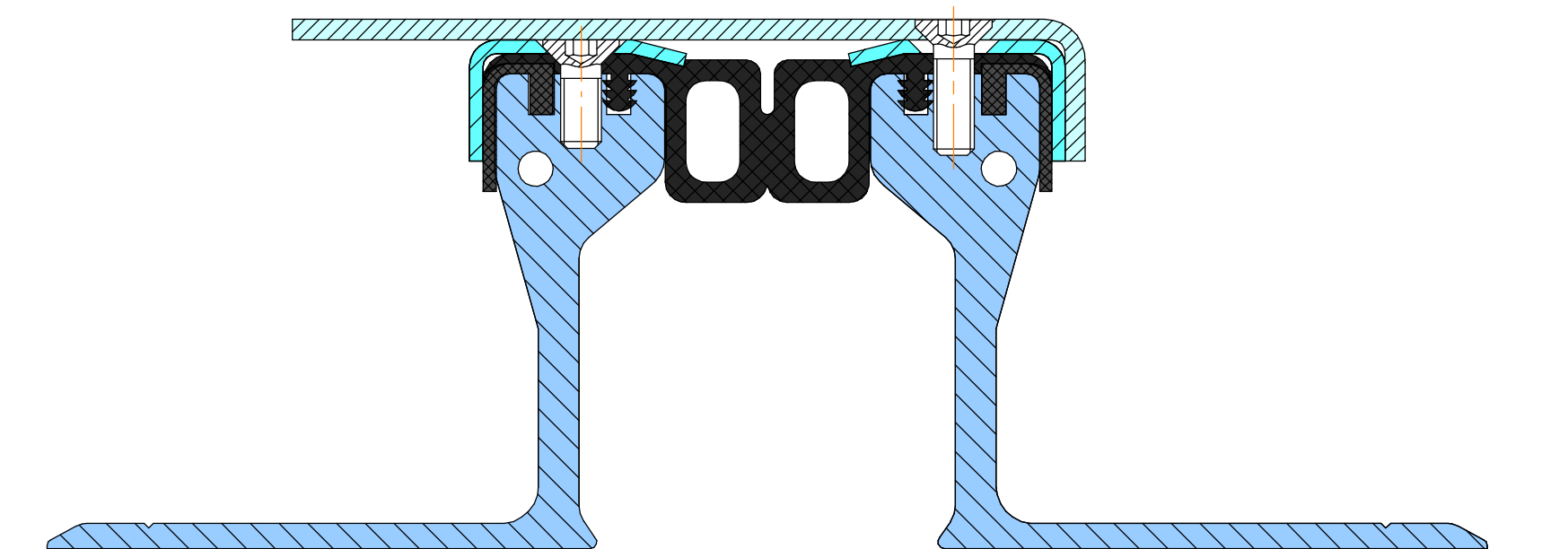
Dewmark Hydro WR 73/50/75/S/F
