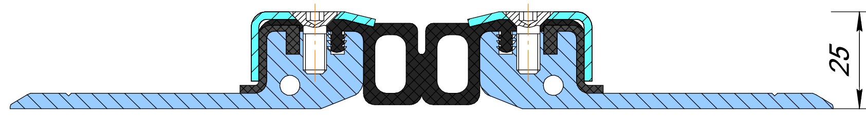
Dewmark Hydro WR 73/50/25/S
