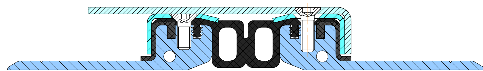
Dewmark Hydro WR 73/50/25/S/F
