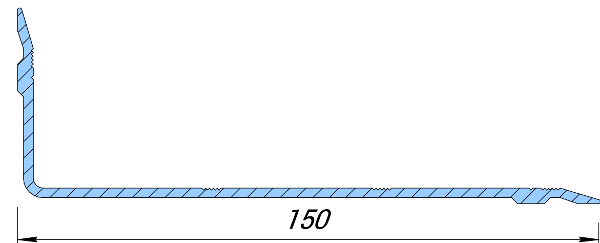
Dewmark Standart SV-E 14/200
