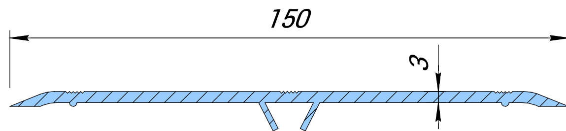
Dewmark Standart SV 14/150
