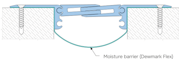
Moisture barrier (Dewmark Flex)
