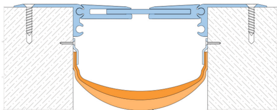
Firebarrier Fireblanket (EI 240)
